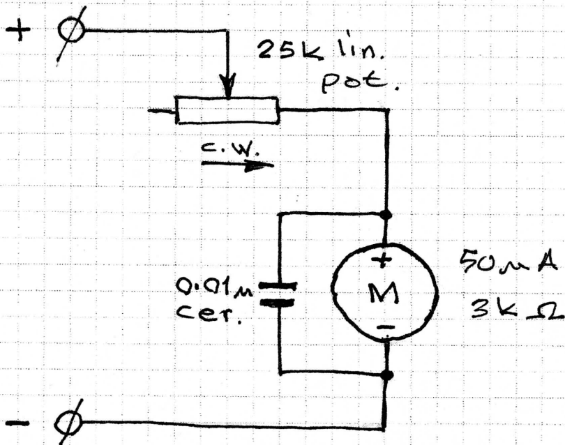
CIRCUIT DIAGRAM
