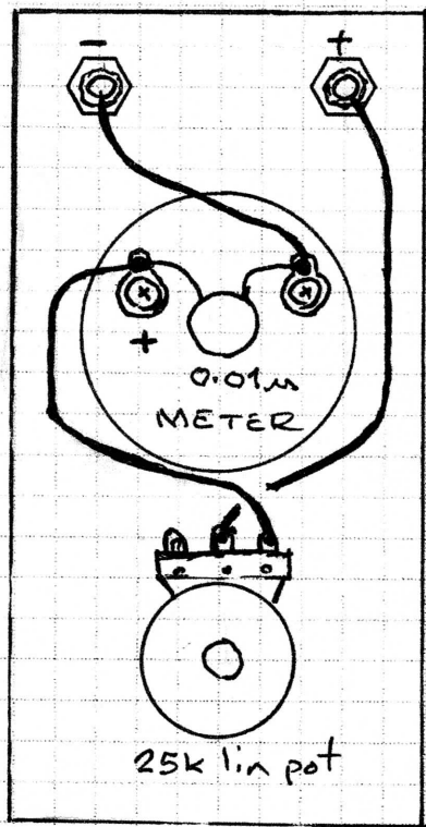
WIRING DETAIL
